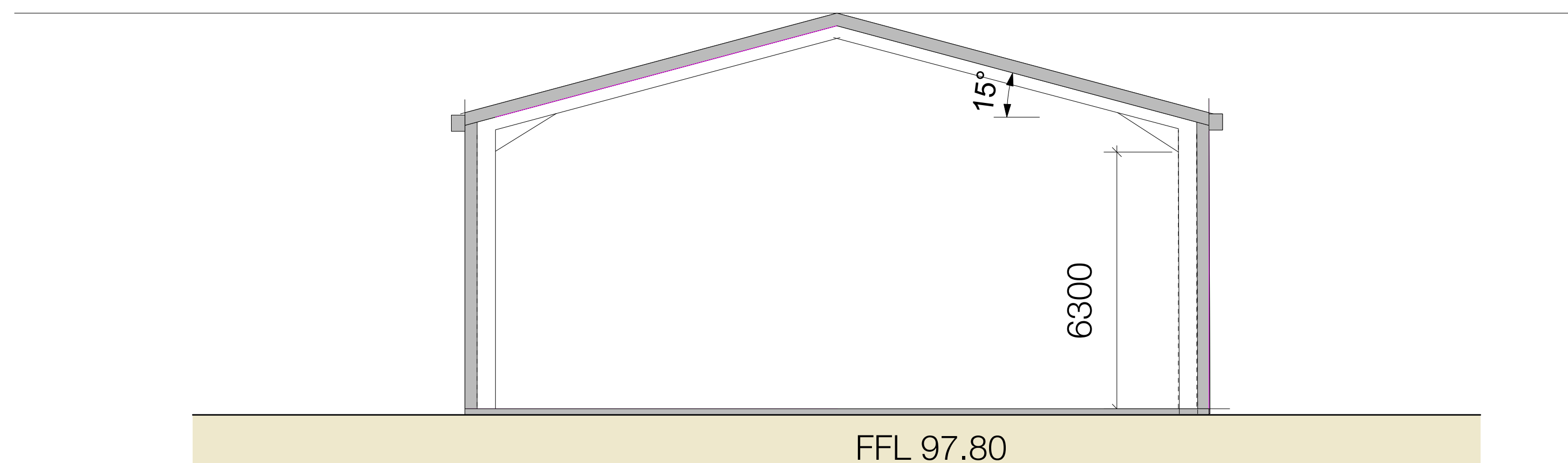
Typical Section
