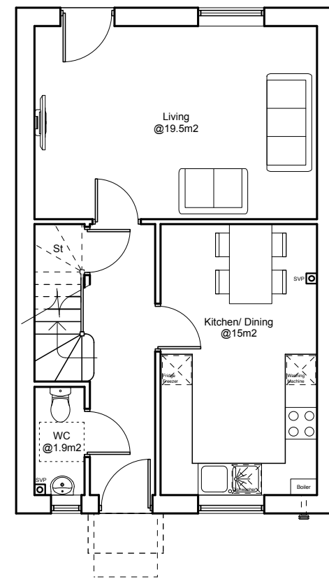
Plot 4 3b5p House @ 95m² Ground Floor Plan
