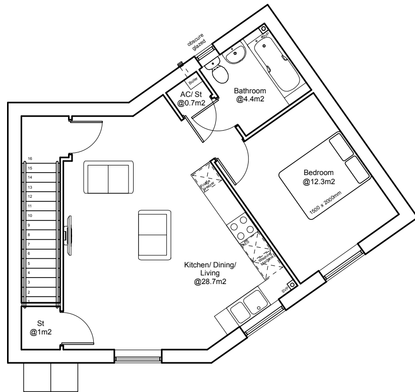
Plot 3 1b2p Flat @ 55m² First Floor Plan
