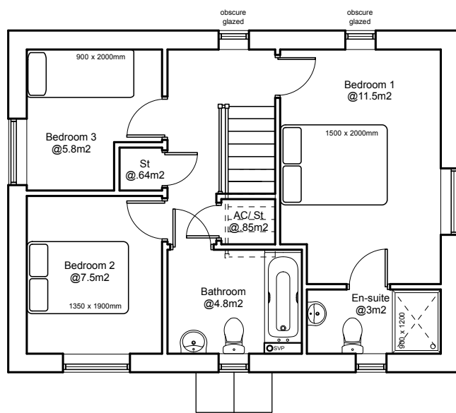
Plot 1 First Floor Plan
