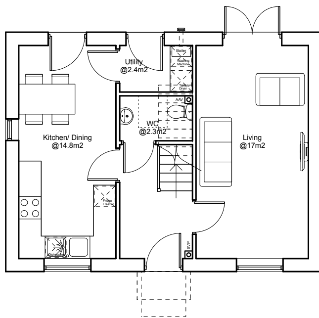
Plot 1 3b5p House @ 88m² Ground Floor Plan
