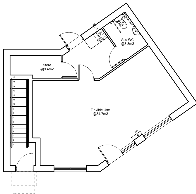
Plot 2 Flexible Use Unit @ 47m² Ground Floor Plan
